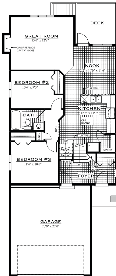
MAIN FLOOR PLAN 996 SQ.FT.
