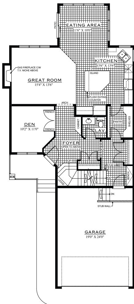
MAIN FLOOR PLAN 1066 SQ.FT.
