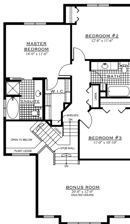
SECOND FLOOR PLAN 1060 SQ.FT.
