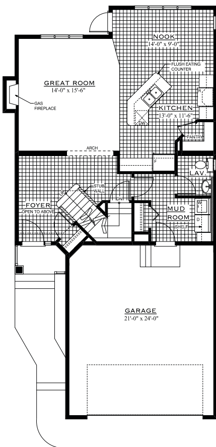
MAIN FLOOR PLAN 875 SQ.FT.
