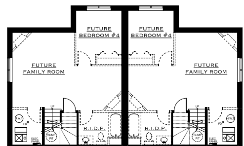
OPTIONAL BASEMENT PLAN 469 SQ.FT.
