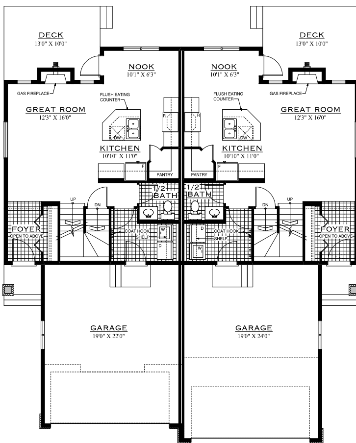
MAIN FLOOR PLAN 650 SQ.FT.
