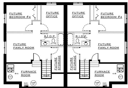
OPTIONAL BASEMENT PLAN 516 SQ.FT.
