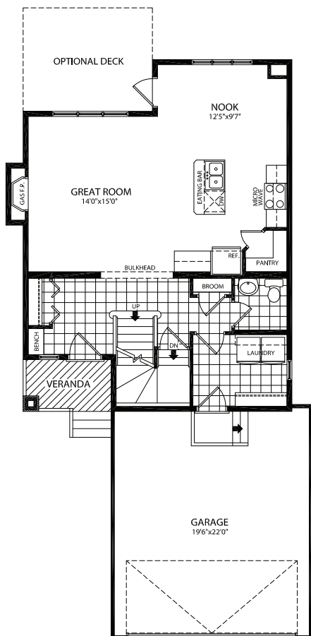
MAIN FLOOR PLAN 779 SQ.FT.
