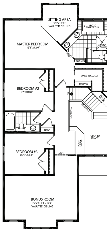
SECOND FLOOR PLAN 1245 SQ.FT.
