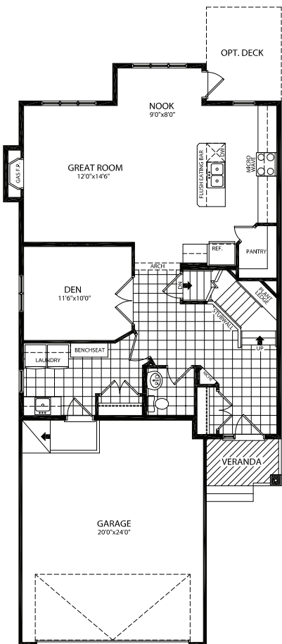
MAIN FLOOR PLAN 1011 SQ.FT.
