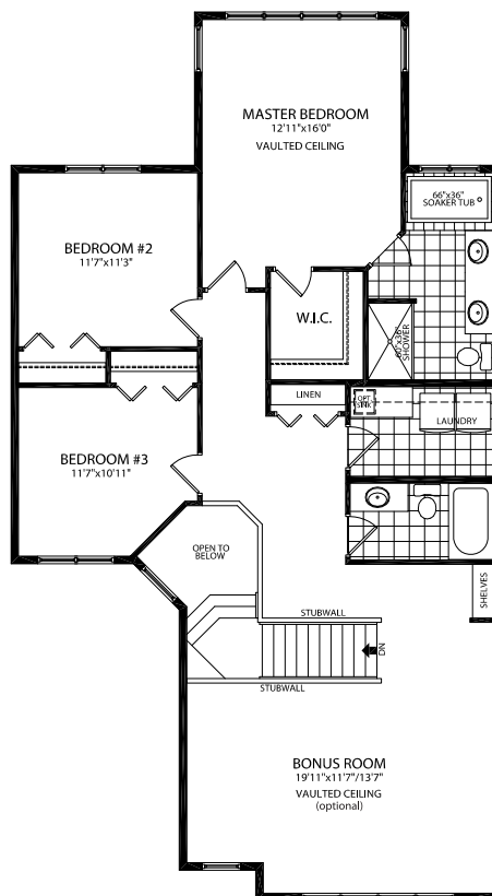
SECOND FLOOR PLAN W/ BONUS ROOM 1332 SQ.FT.
