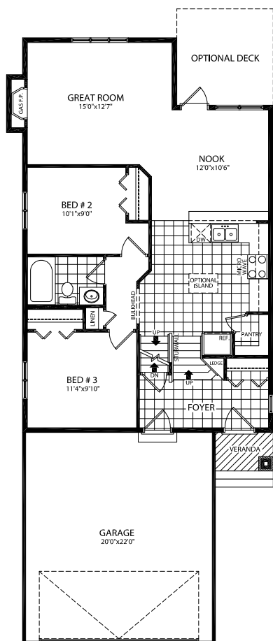
MAIN FLOOR PLAN 996 SQ.FT.
