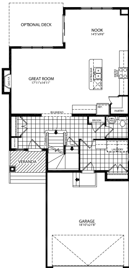
MAIN FLOOR PLAN 909 SQ.FT.
