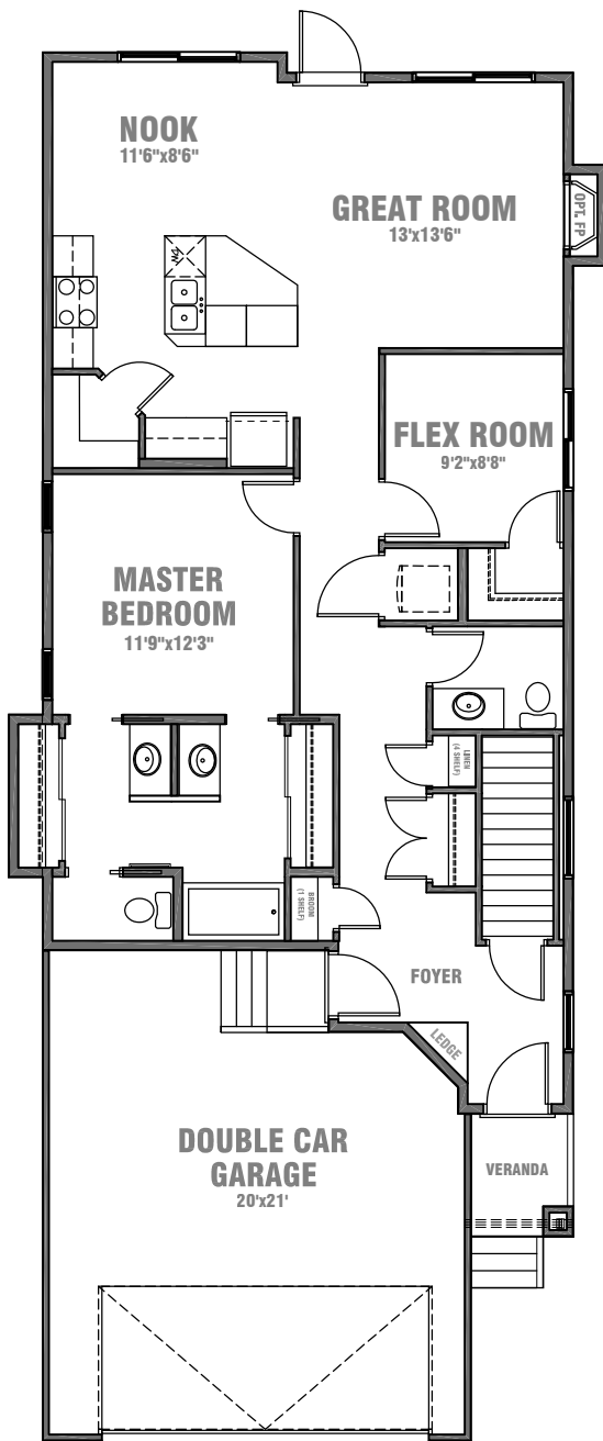
MAIN FLOOR PLAN 1217 SQ.FT.
