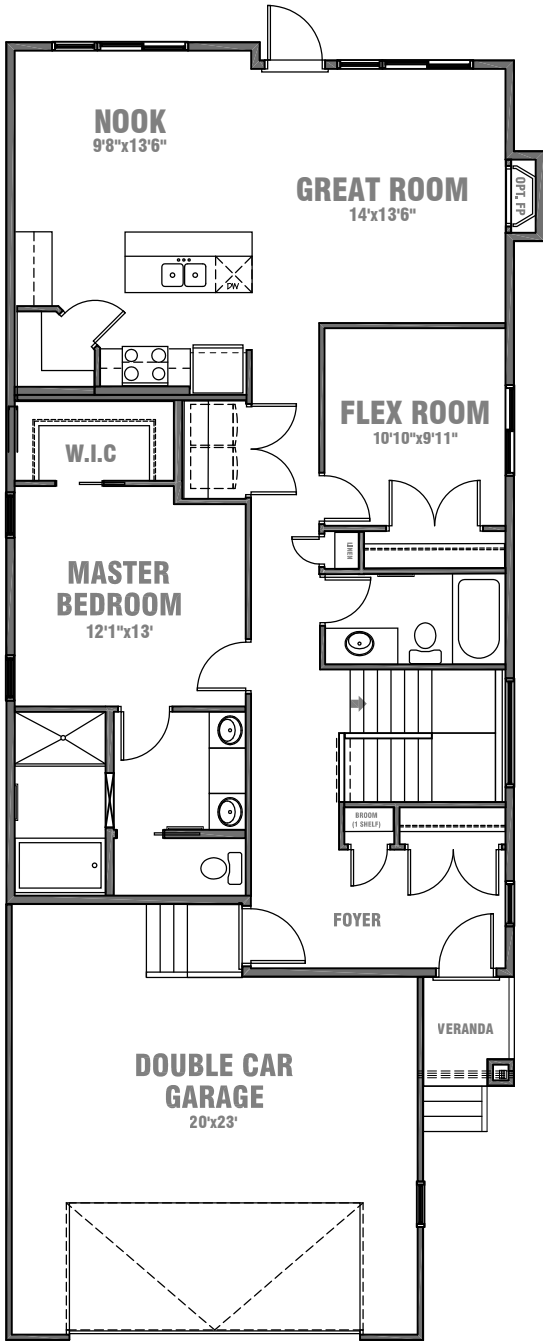
MAIN FLOOR PLAN 1384 SQ.FT.
