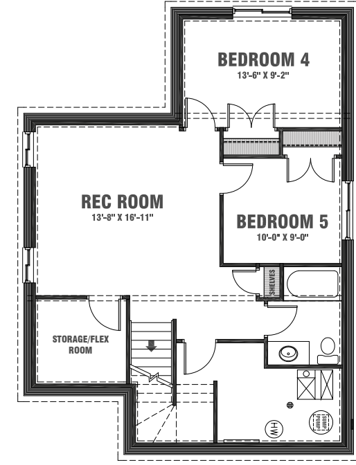
BASEMENT DEVELOPMENT 638 SQ.FT.
