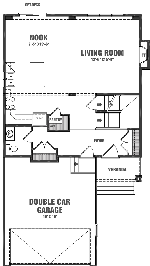
MAIN FLOOR PLAN 818 SQ.FT.
