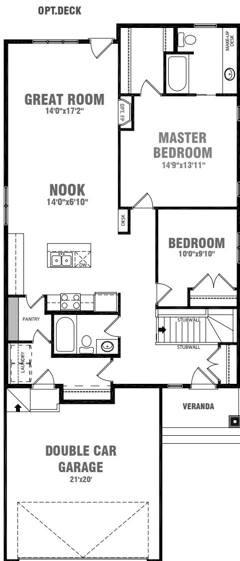
MAIN FLOOR 1365 SQ.FT.
