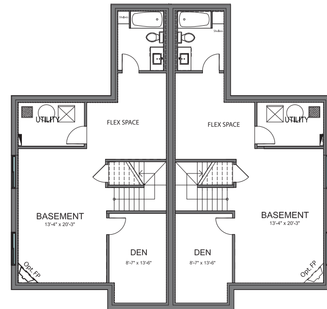
Optional Basement Development FINISHED AREA 667 SQ.FT. UNFINISHED AREA 66 SQ.FT.
