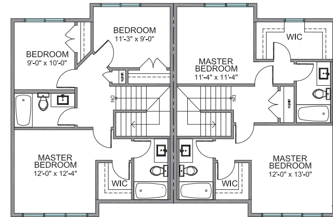
SECOND FLOOR 3 Bedroom Option 707 SQ.FT.
