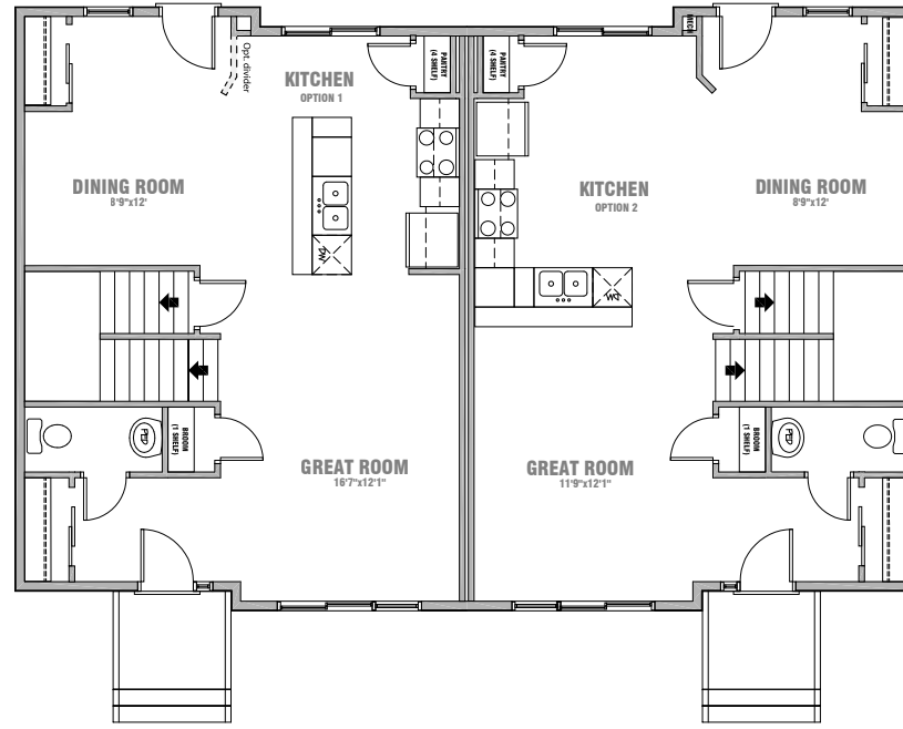
MAIN FLOOR 685 SQ.FT.
