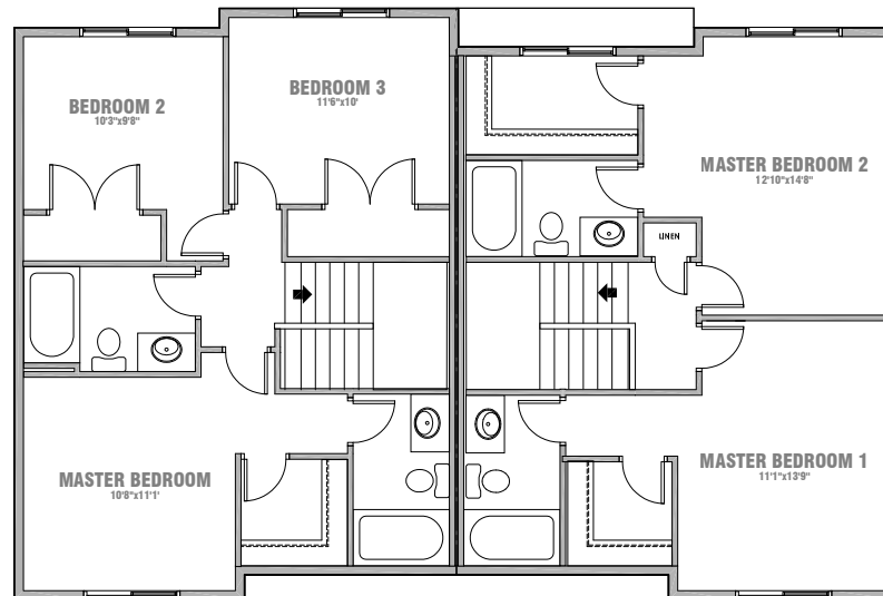
SECOND FLOOR 3 Bedroom 624 SQ.FT.
